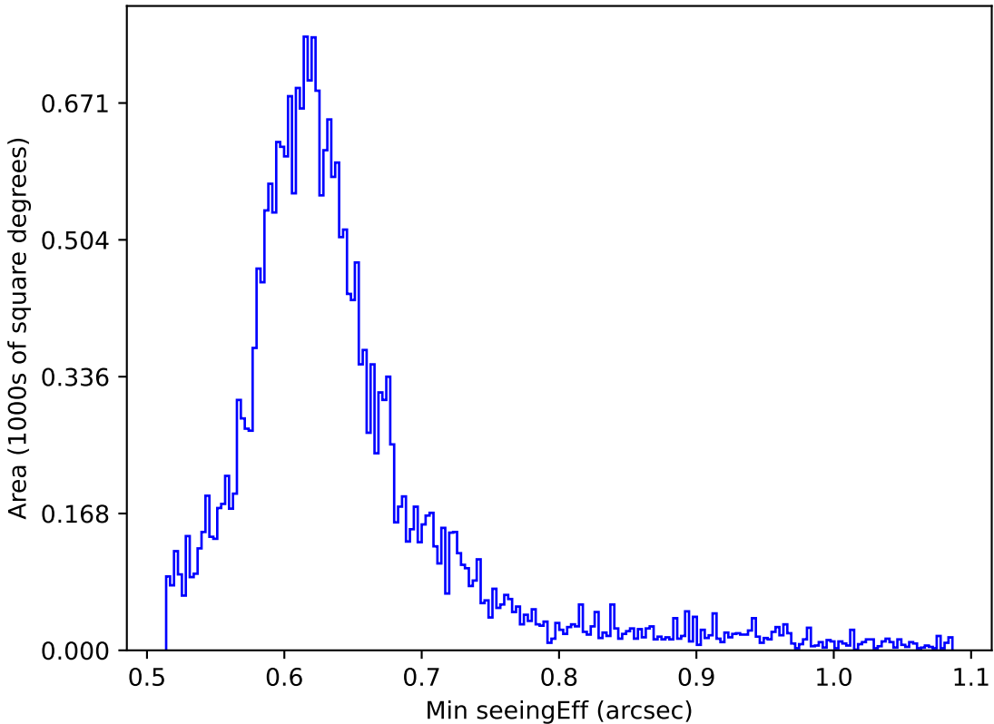
too_elab_r64_d3_griz_v3.4_10yrs All sky r band: Min seeingEff
