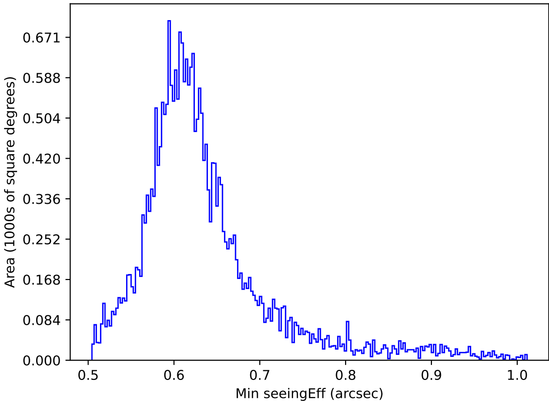
too_elab_r64_d3_griz_v3.4_10yrs All sky i band: Min seeingEff
