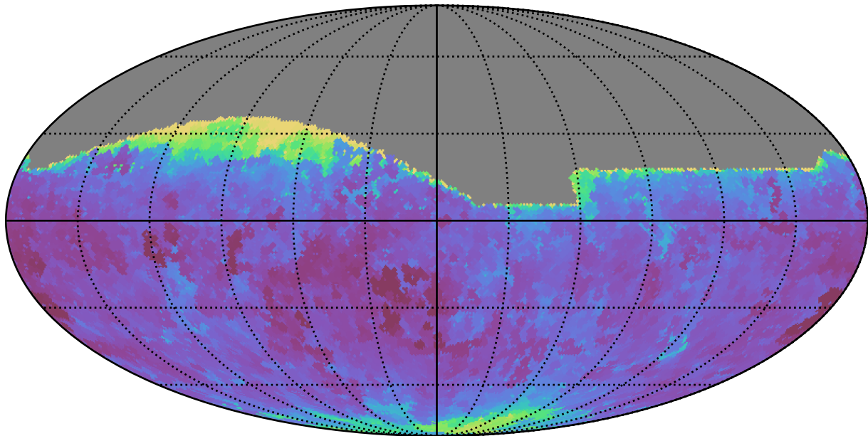
too_elab_r64_d3_griz_v3.4_10yrs All sky g band: Min seeingEff
