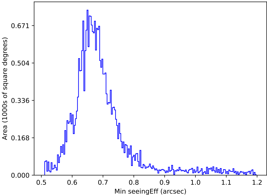
too_elab_r64_d3_griz_v3.4_10yrs All sky g band: Min seeingEff
