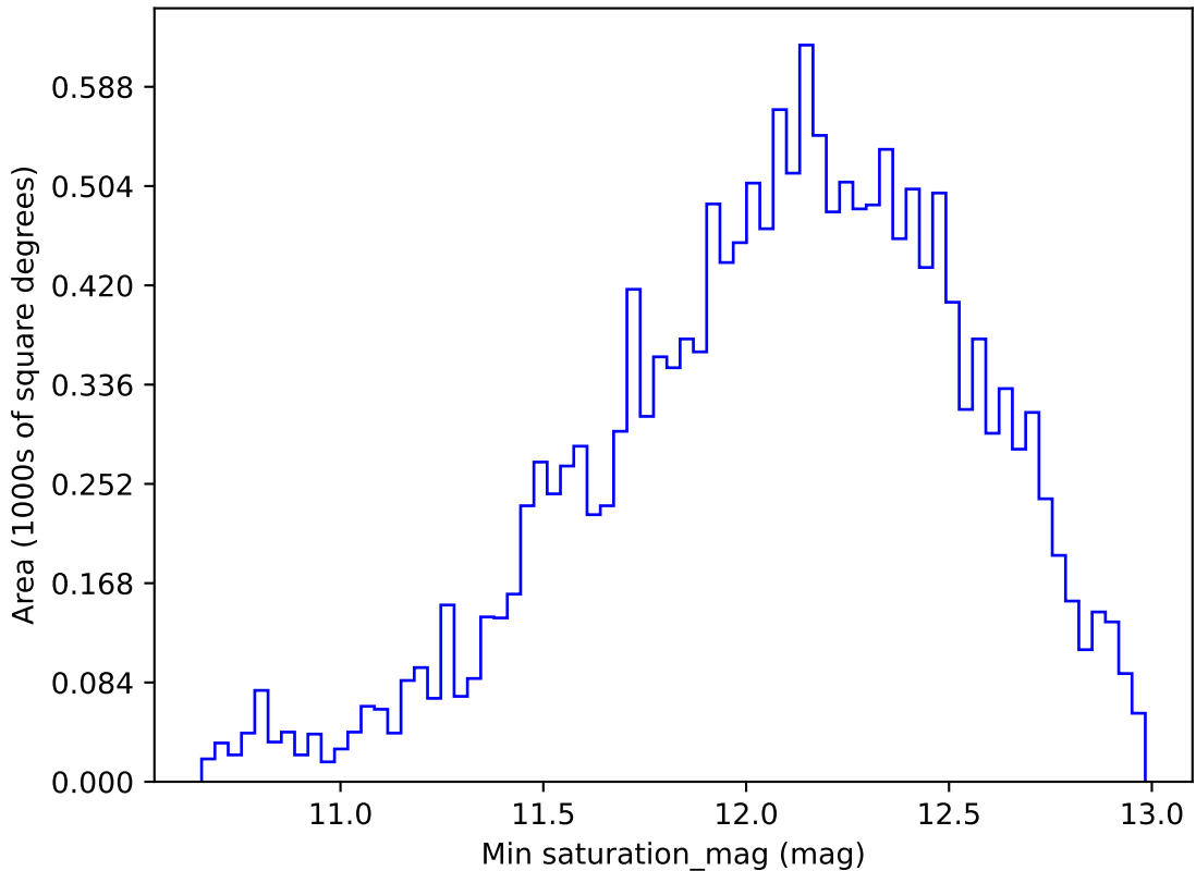
too_elab_r64_d3_griz_v3.4_10yrs WFD z band: Min saturation_mag
