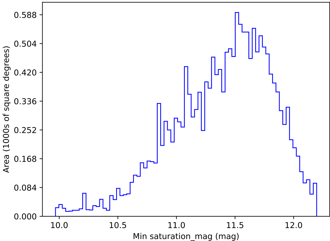
too_elab_r64_d3_griz_v3.4_10yrs WFD u band: Min saturation_mag
