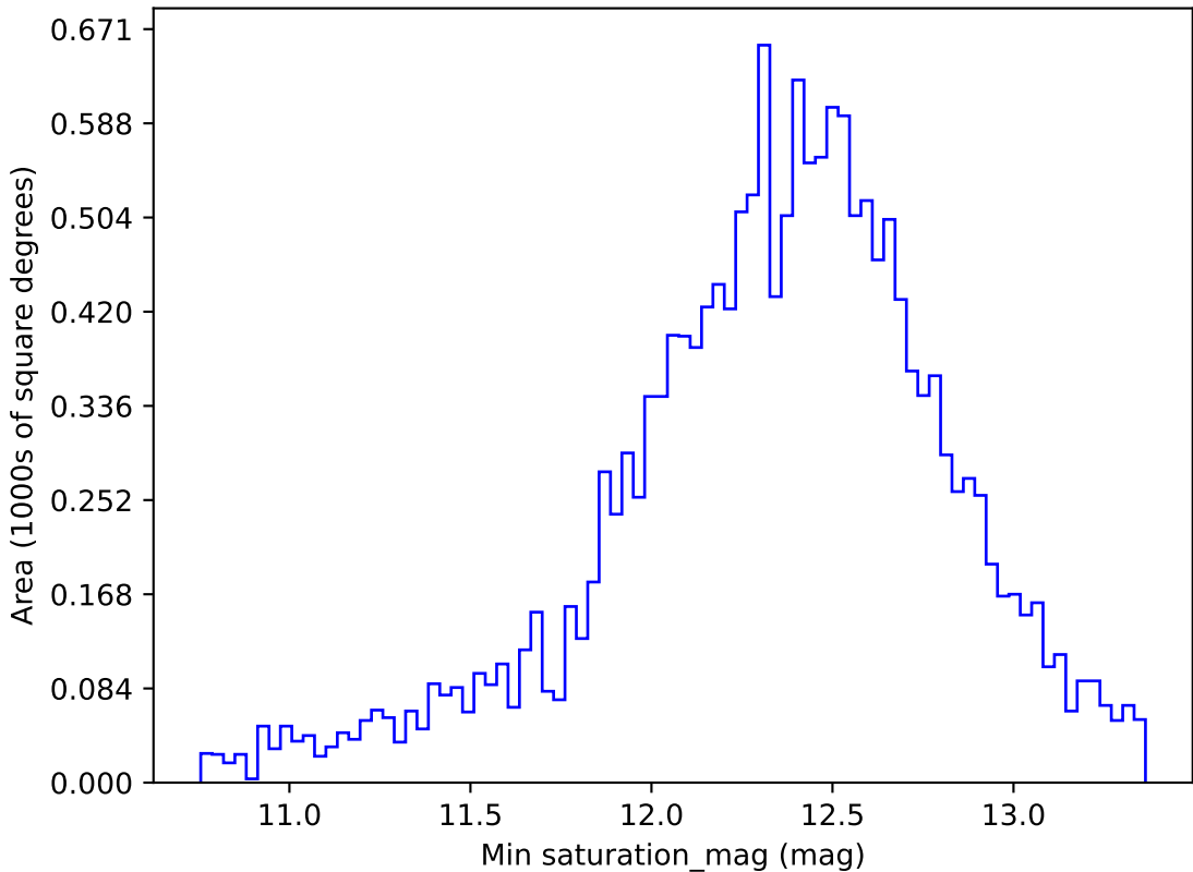
too_elab_r64_d3_griz_v3.4_10yrs WFD i band: Min saturation_mag
