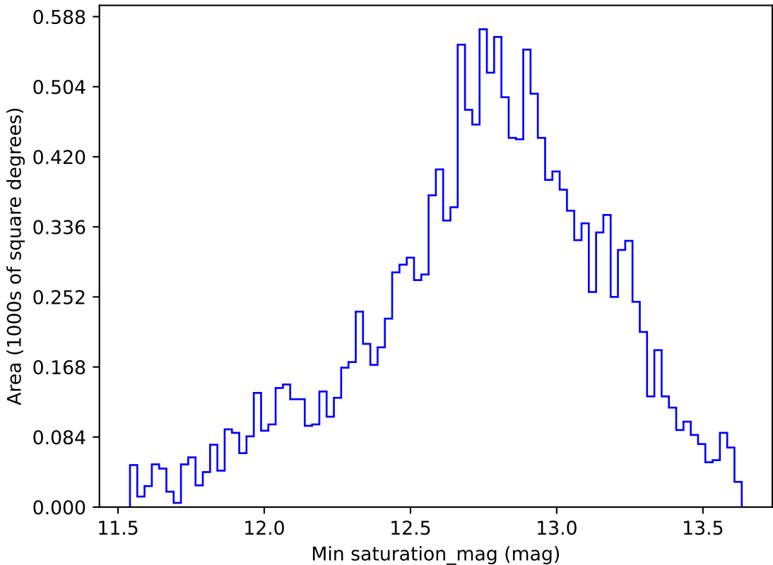
too_elab_r64_d3_griz_v3.4_10yrs WFD g band: Min saturation_mag
