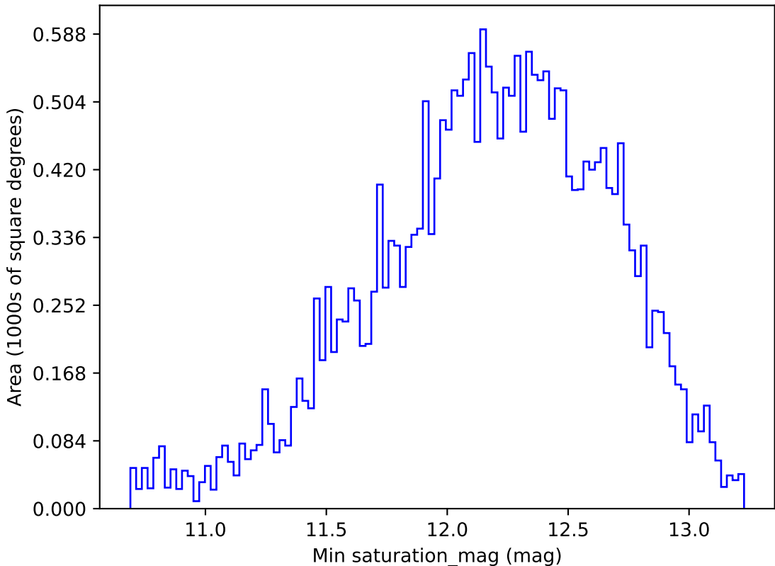
too_elab_r64_d3_griz_v3.4_10yrs All sky z band: Min saturation_mag
