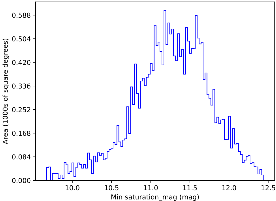
too_elab_r64_d3_griz_v3.4_10yrs All sky y band: Min saturation_mag
