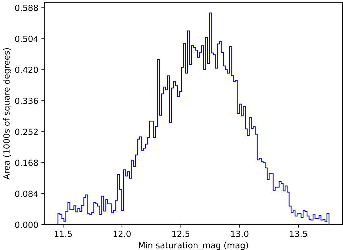
too_elab_r64_d3_griz_v3.4_10yrs All sky r band: Min saturation_mag
