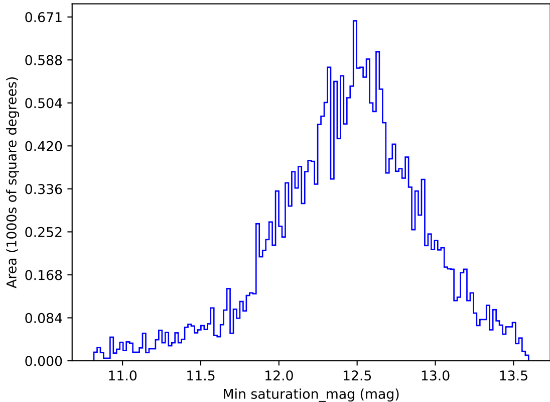
too_elab_r64_d3_griz_v3.4_10yrs All sky i band: Min saturation_mag
