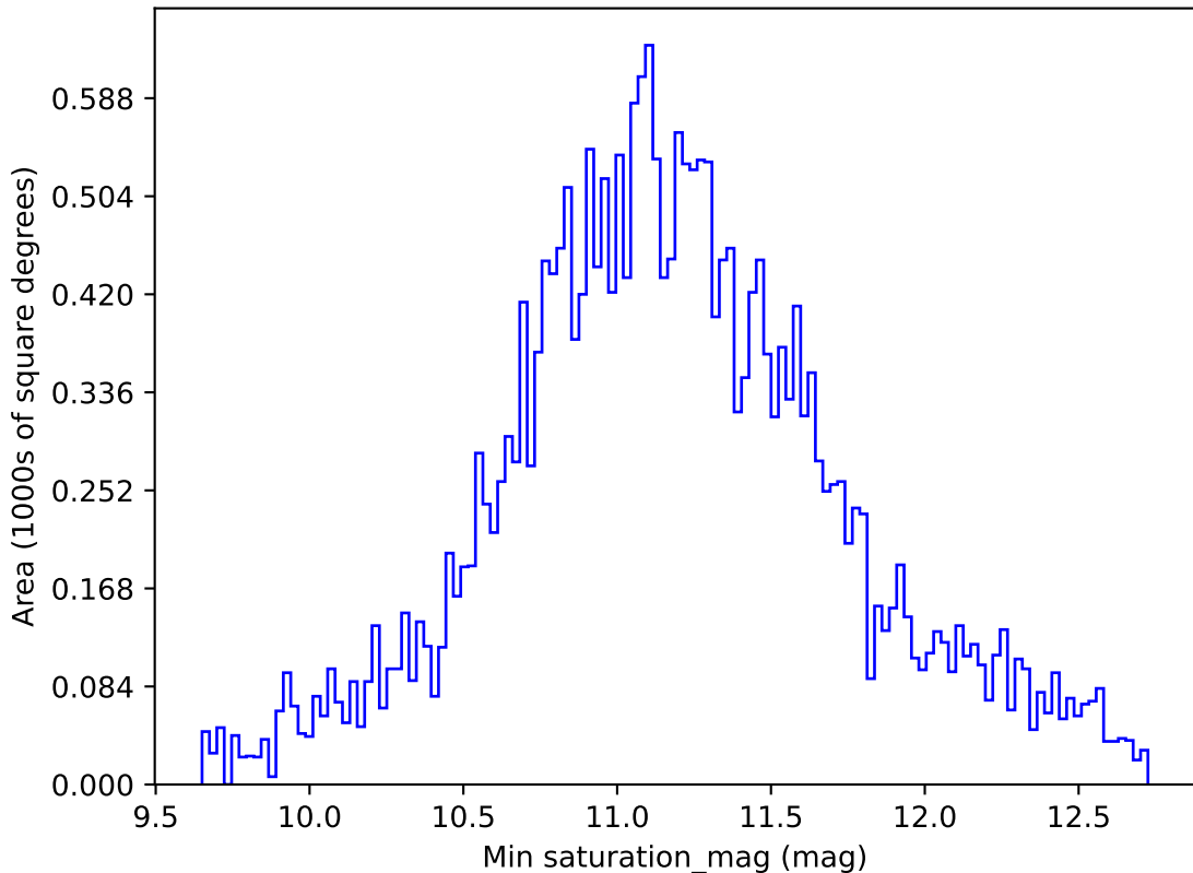
too_elab_r64_d3_griz_v3.4_10yrs All sky all bands: Min saturation_mag
