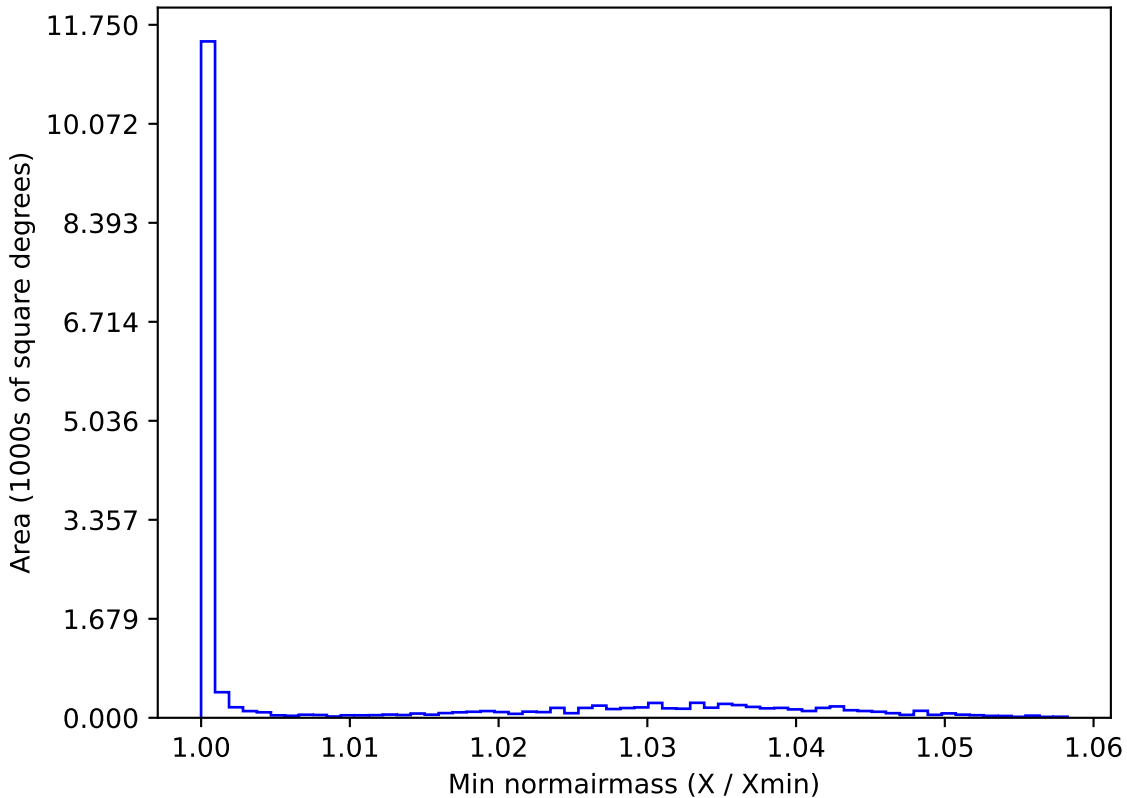
too_elab_r64_d3_griz_v3.4_10yrs WFD u band: Min normairmass
