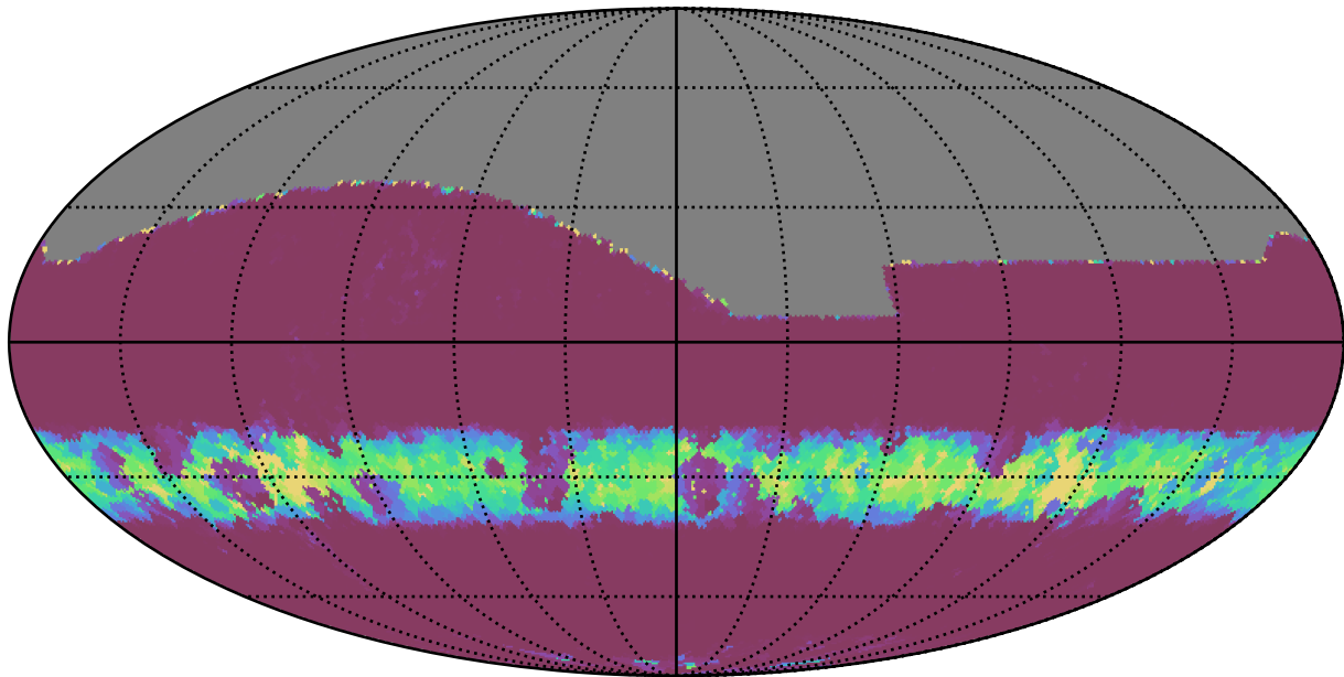
too_elab_r64_d3_griz_v3.4_10yrs All sky i band: Min normairmass
