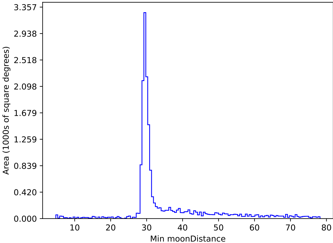
too_elab_r64_d3_griz_v3.4_10yrs WFD z band: Min moonDistance
