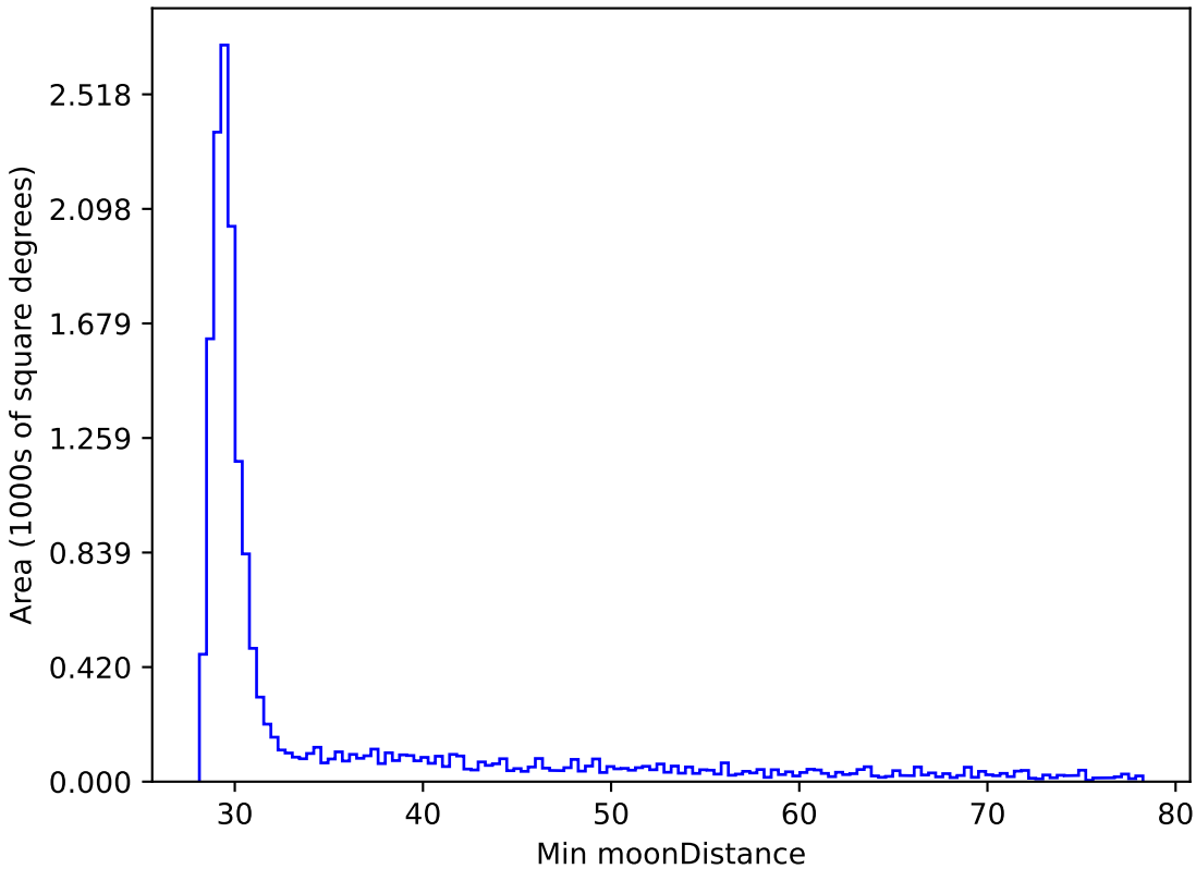
too_elab_r64_d3_griz_v3.4_10yrs WFD y band: Min moonDistance
