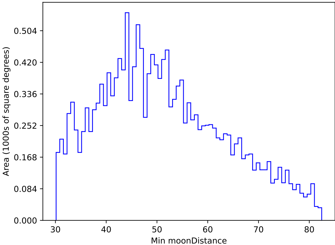
too_elab_r64_d3_griz_v3.4_10yrs WFD u band: Min moonDistance
