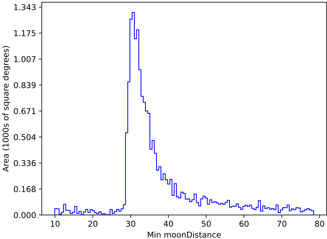
too_elab_r64_d3_griz_v3.4_10yrs WFD r band: Min moonDistance
