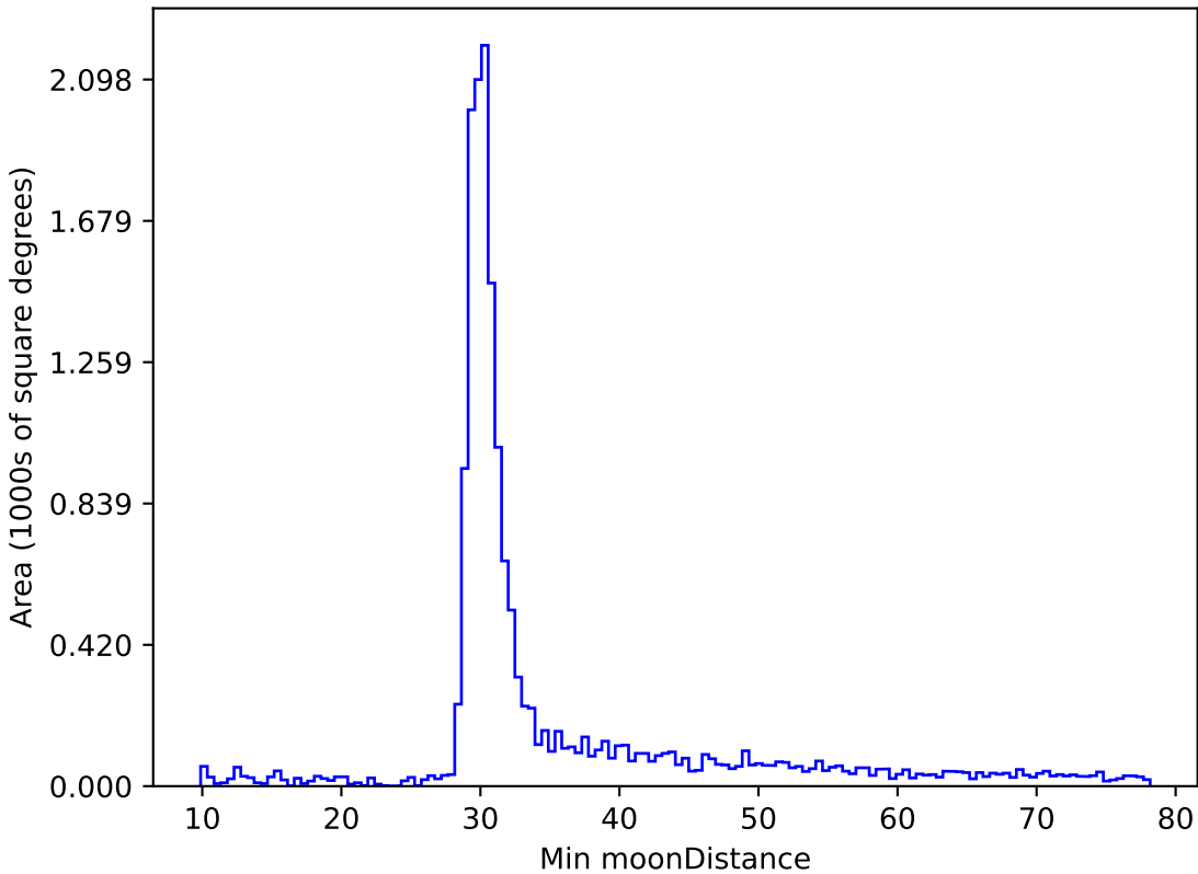
too_elab_r64_d3_griz_v3.4_10yrs WFD i band: Min moonDistance
