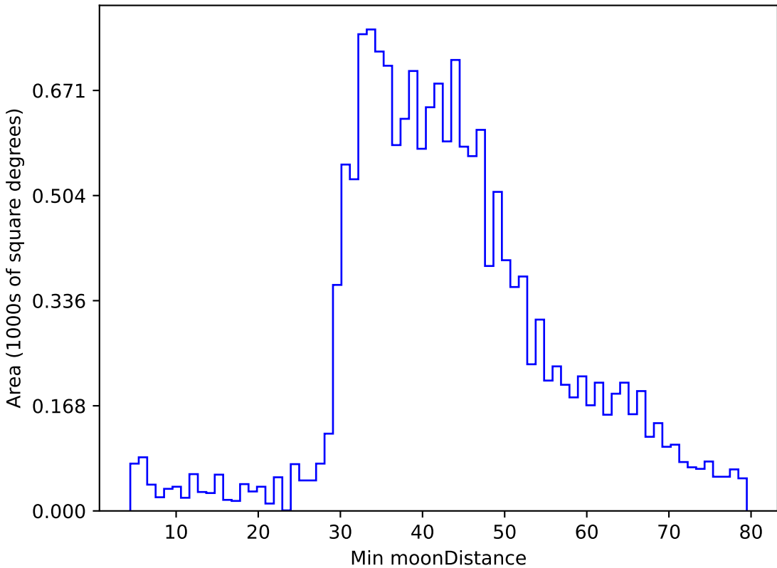
too_elab_r64_d3_griz_v3.4_10yrs WFD g band: Min moonDistance
