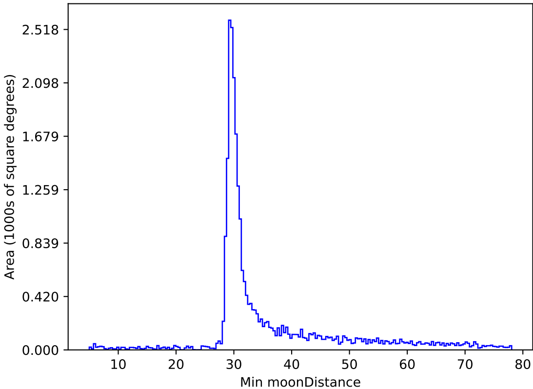
too_elab_r64_d3_griz_v3.4_10yrs All sky z band: Min moonDistance
