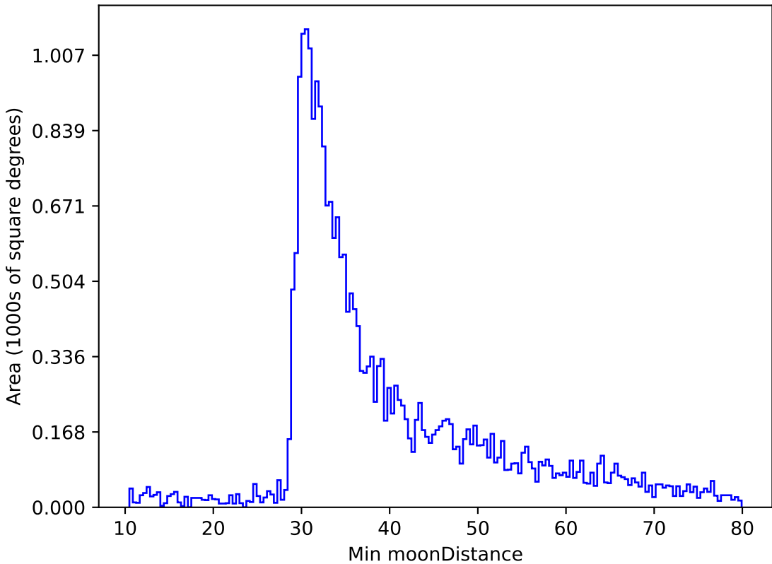
too_elab_r64_d3_griz_v3.4_10yrs All sky r band: Min moonDistance
