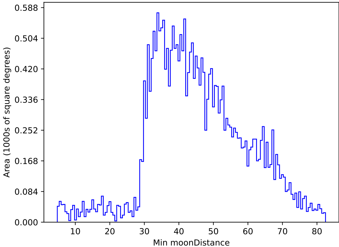
too_elab_r64_d3_griz_v3.4_10yrs All sky g band: Min moonDistance
