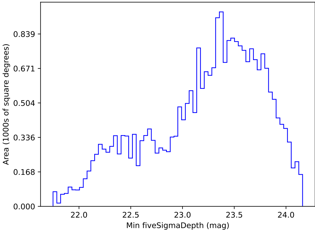
too_elab_r64_d3_griz_v3.4_10yrs Yr 1 r band: Min fiveSigmaDepth
