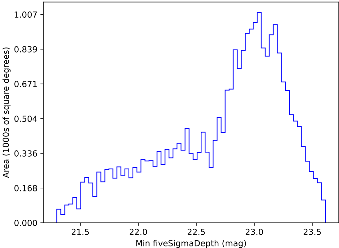
too_elab_r64_d3_griz_v3.4_10yrs Yr 1 i band: Min fiveSigmaDepth
