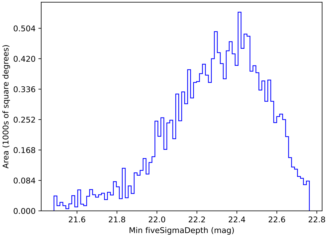
too_elab_r64_d3_griz_v3.4_10yrs WFD u band: Min fiveSigmaDepth
