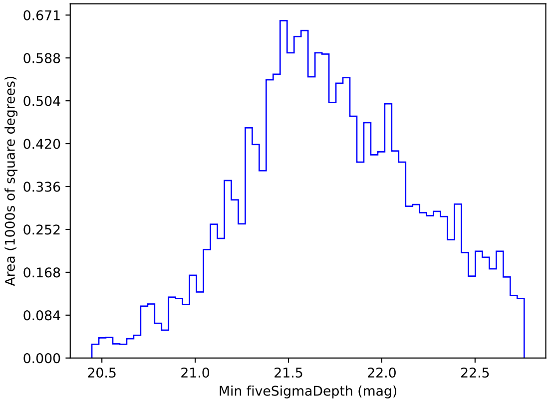
too_elab_r64_d3_griz_v3.4_10yrs WFD i band: Min fiveSigmaDepth
