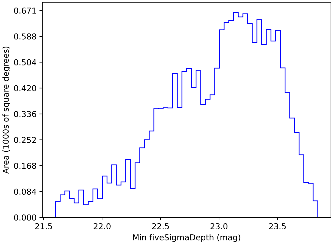
too_elab_r64_d3_griz_v3.4_10yrs WFD g band: Min fiveSigmaDepth
