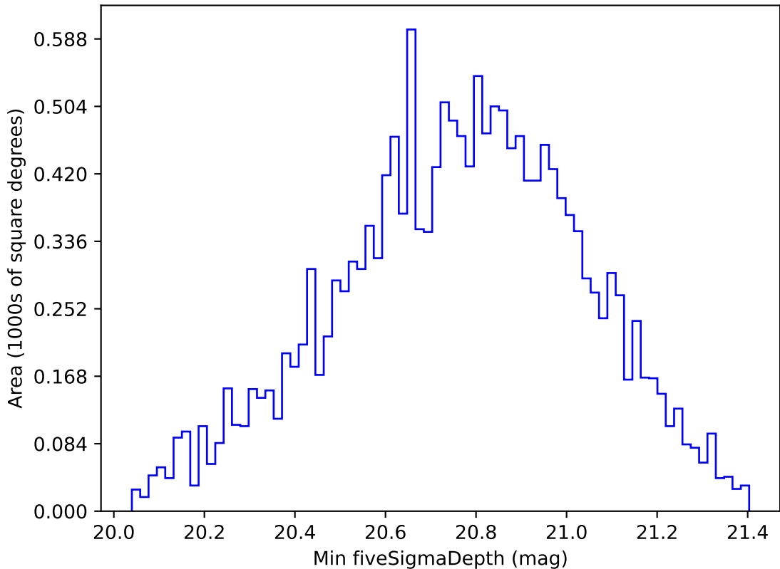
too_elab_r64_d3_griz_v3.4_10yrs WFD all bands: Min fiveSigmaDepth
