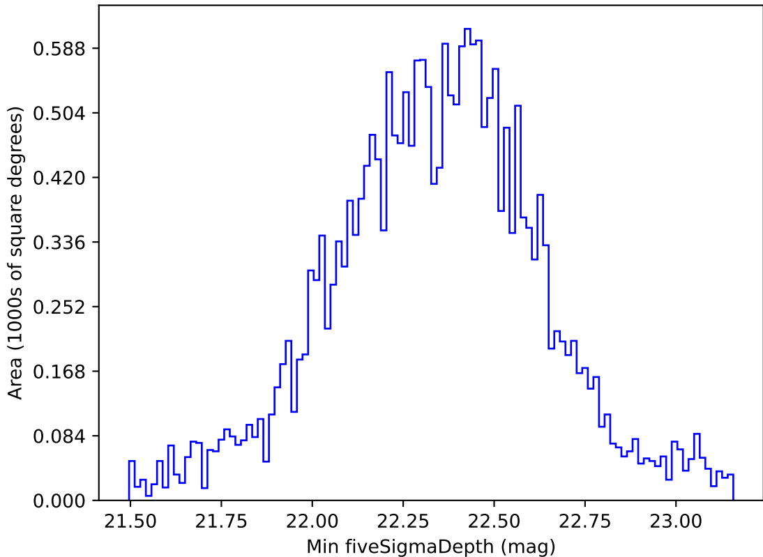
too_elab_r64_d3_griz_v3.4_10yrs All sky u band: Min fiveSigmaDepth
