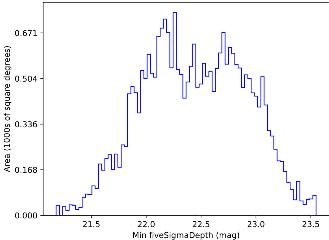
too_elab_r64_d3_griz_v3.4_10yrs All sky r band: Min fiveSigmaDepth
