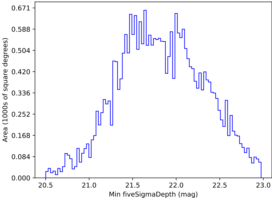
too_elab_r64_d3_griz_v3.4_10yrs All sky i band: Min fiveSigmaDepth
