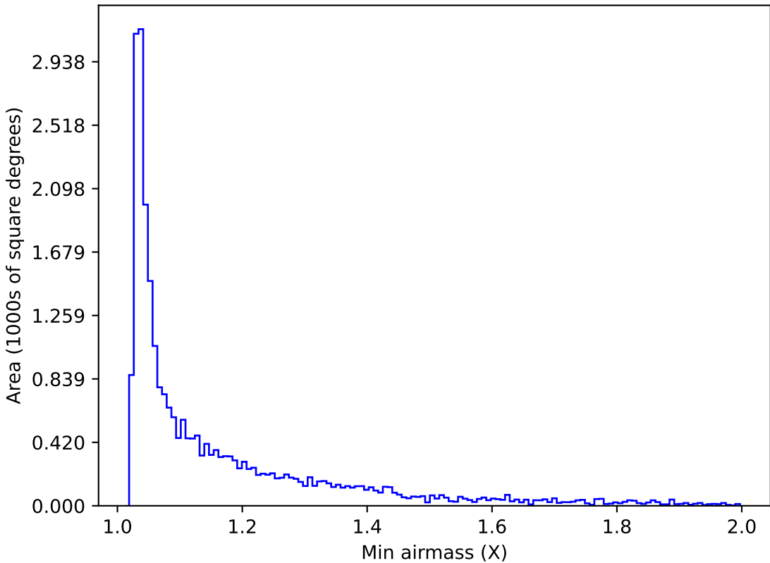
too_elab_r64_d3_griz_v3.4_10yrs Yr 1 i band: Min airmass
