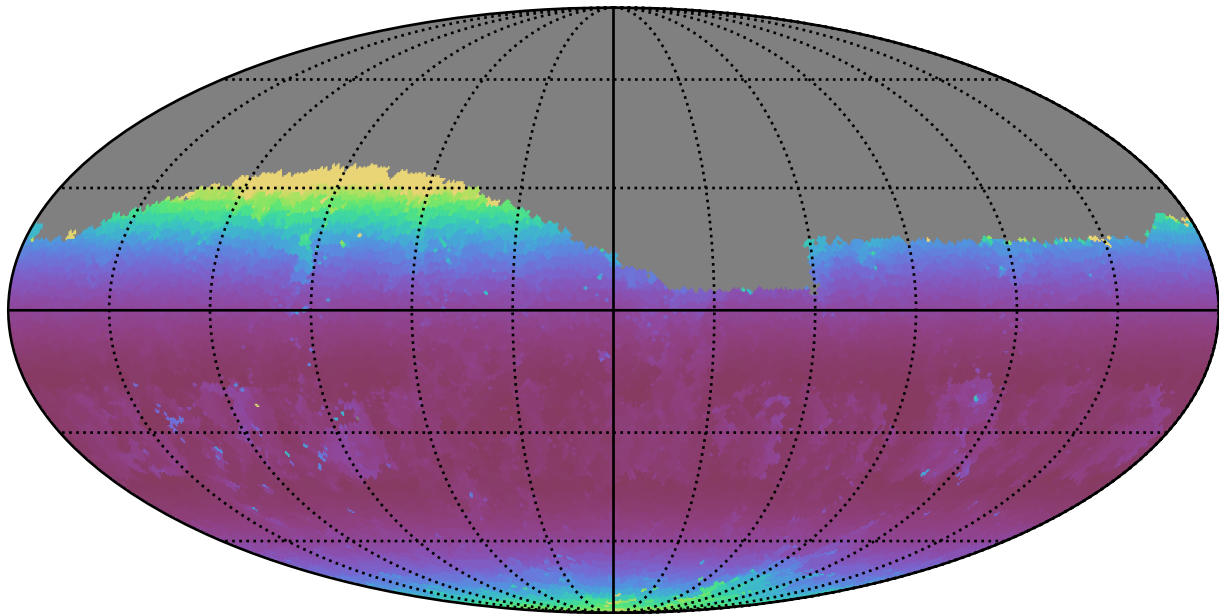
too_elab_r64_d3_griz_v3.4_10yrs Yr 1 g band: Min airmass
