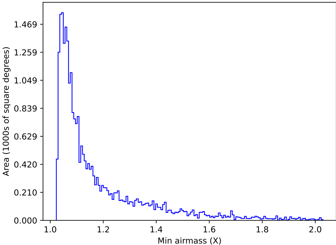
too_elab_r64_d3_griz_v3.4_10yrs Yr 1 g band: Min airmass
