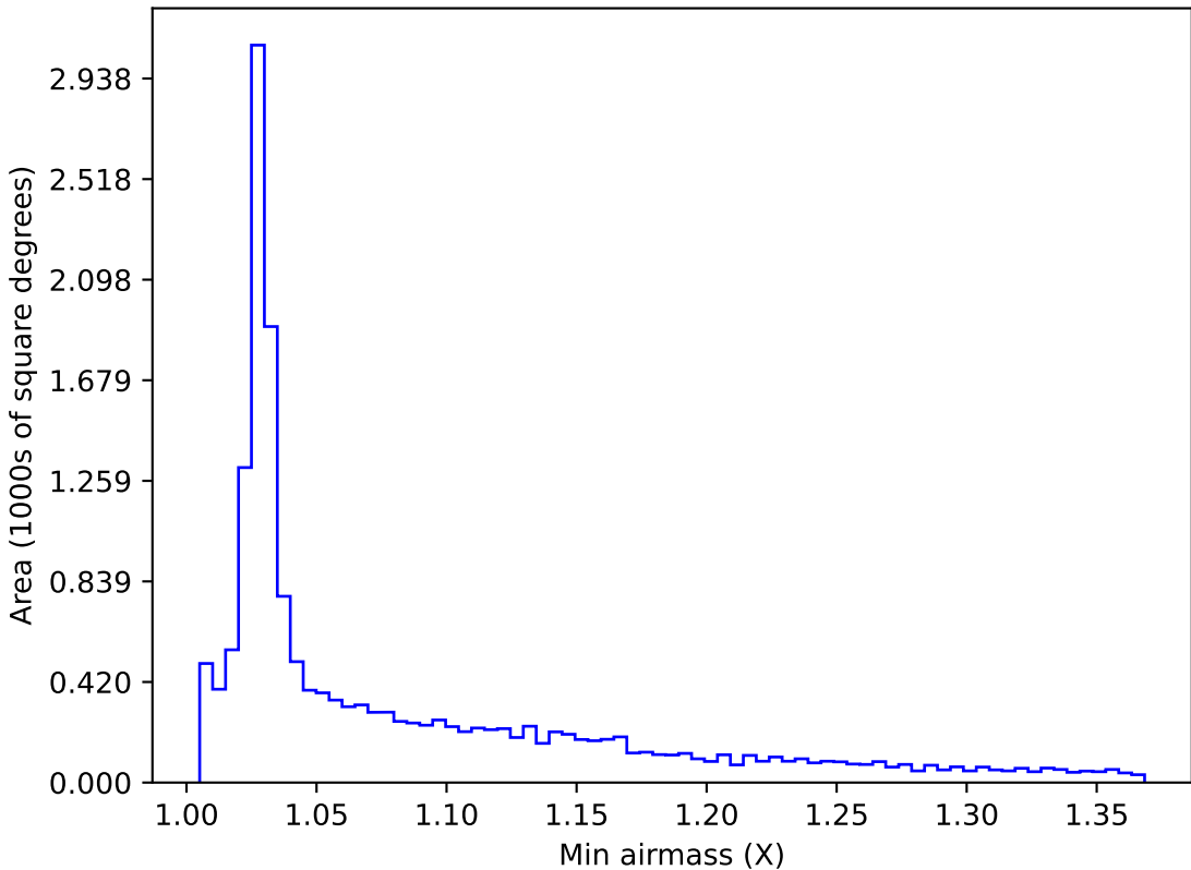
too_elab_r64_d3_griz_v3.4_10yrs WFD z band: Min airmass
