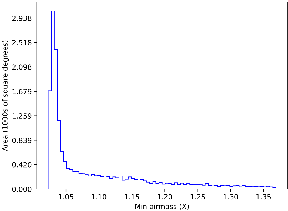
too_elab_r64_d3_griz_v3.4_10yrs WFD y band: Min airmass
