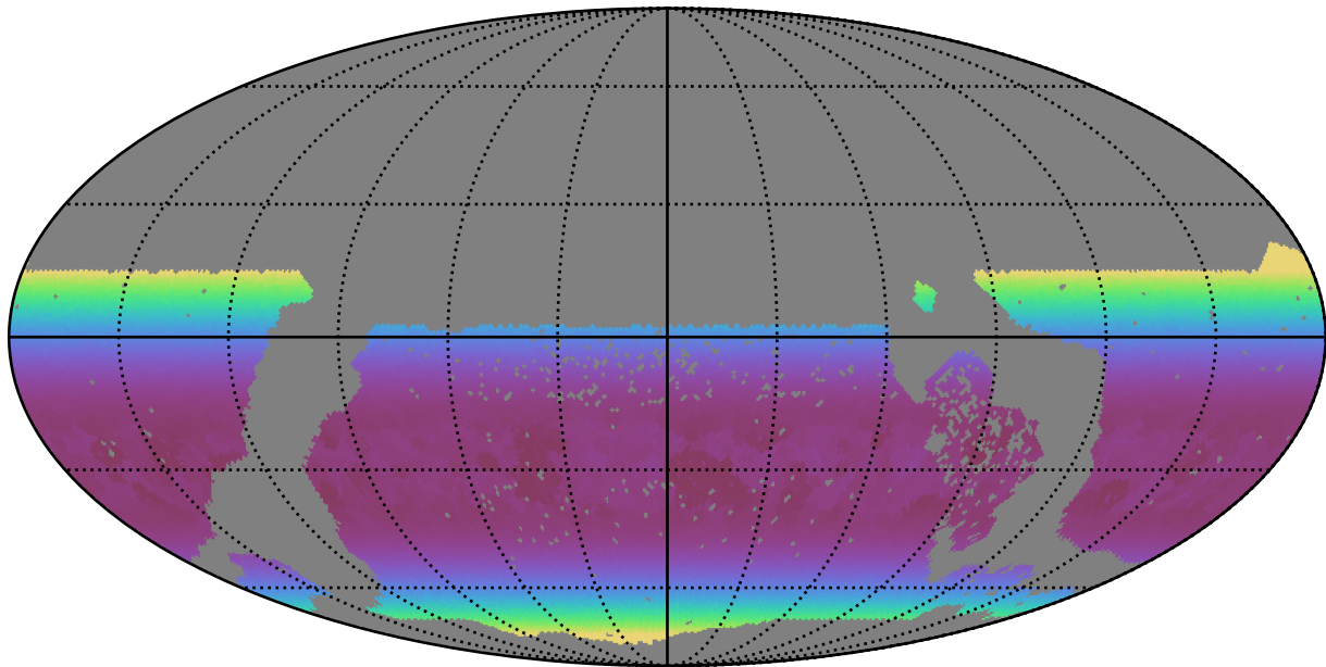
too_elab_r64_d3_griz_v3.4_10yrs WFD r band: Min airmass
