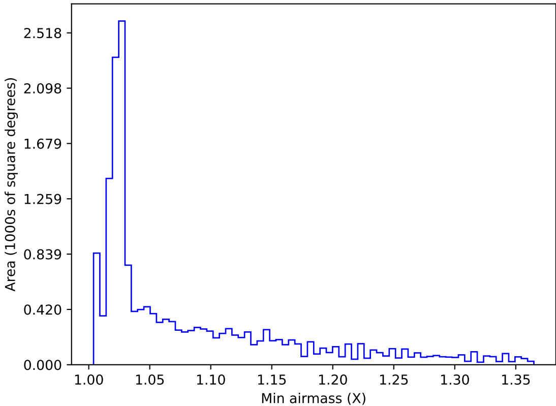
too_elab_r64_d3_griz_v3.4_10yrs WFD all bands: Min airmass
