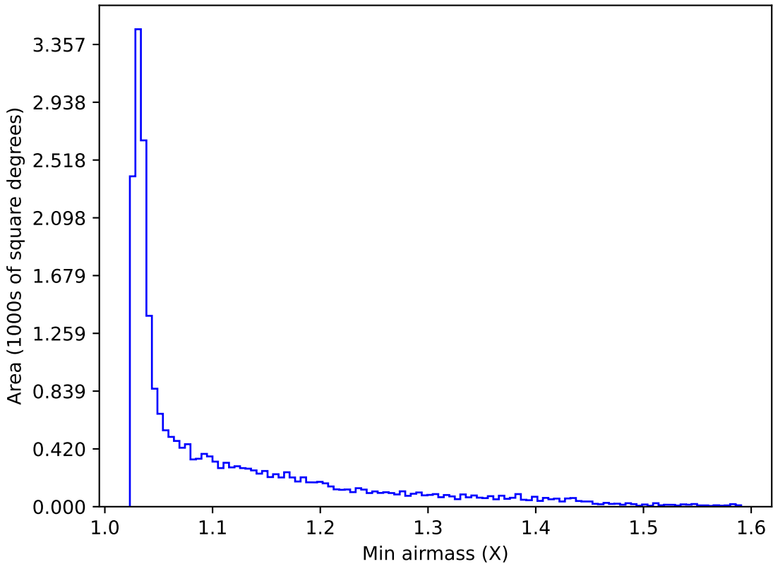
too_elab_r64_d3_griz_v3.4_10yrs All sky y band: Min airmass
