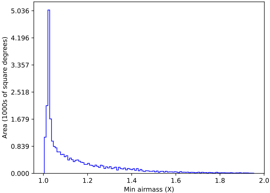
too_elab_r64_d3_griz_v3.4_10yrs All sky all bands: Min airmass
