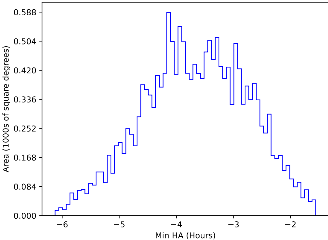
too_elab_r64_d3_griz_v3.4_10yrs WFD y band: Min HA
