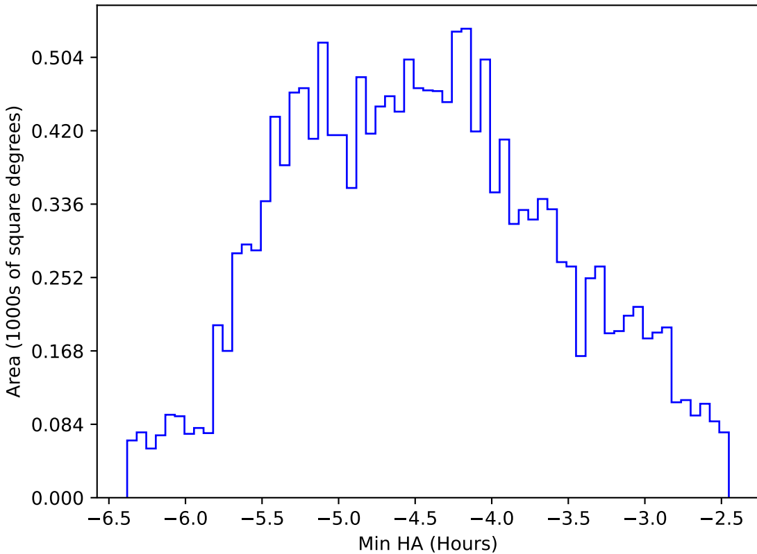
too_elab_r64_d3_griz_v3.4_10yrs WFD r band: Min HA
