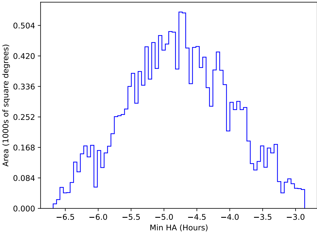
too_elab_r64_d3_griz_v3.4_10yrs WFD all bands: Min HA
