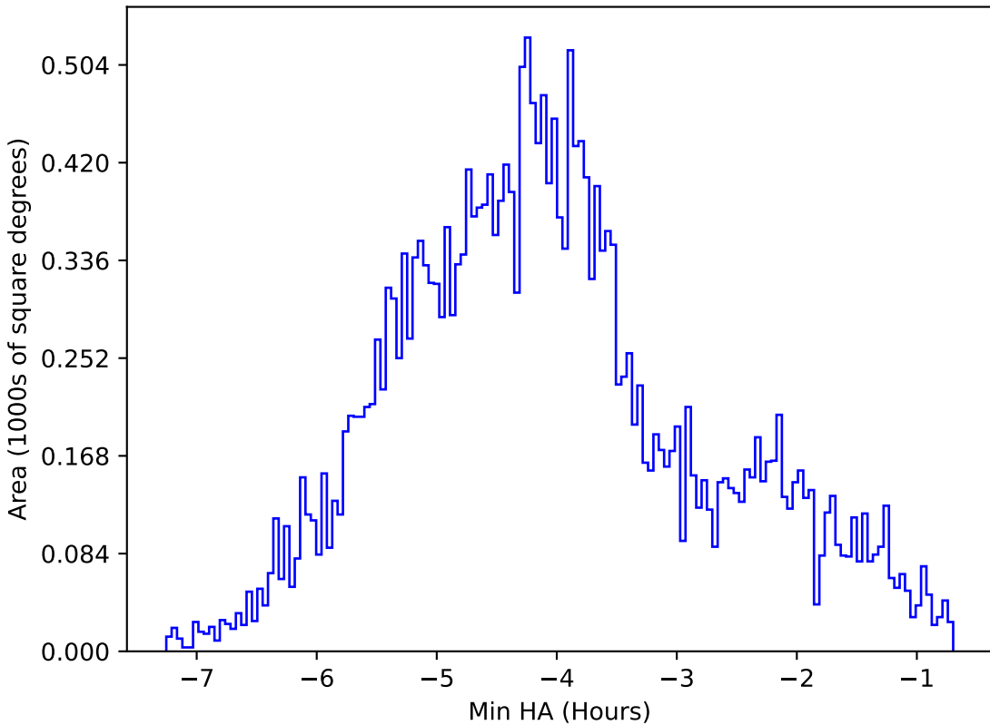
too_elab_r64_d3_griz_v3.4_10yrs All sky z band: Min HA
