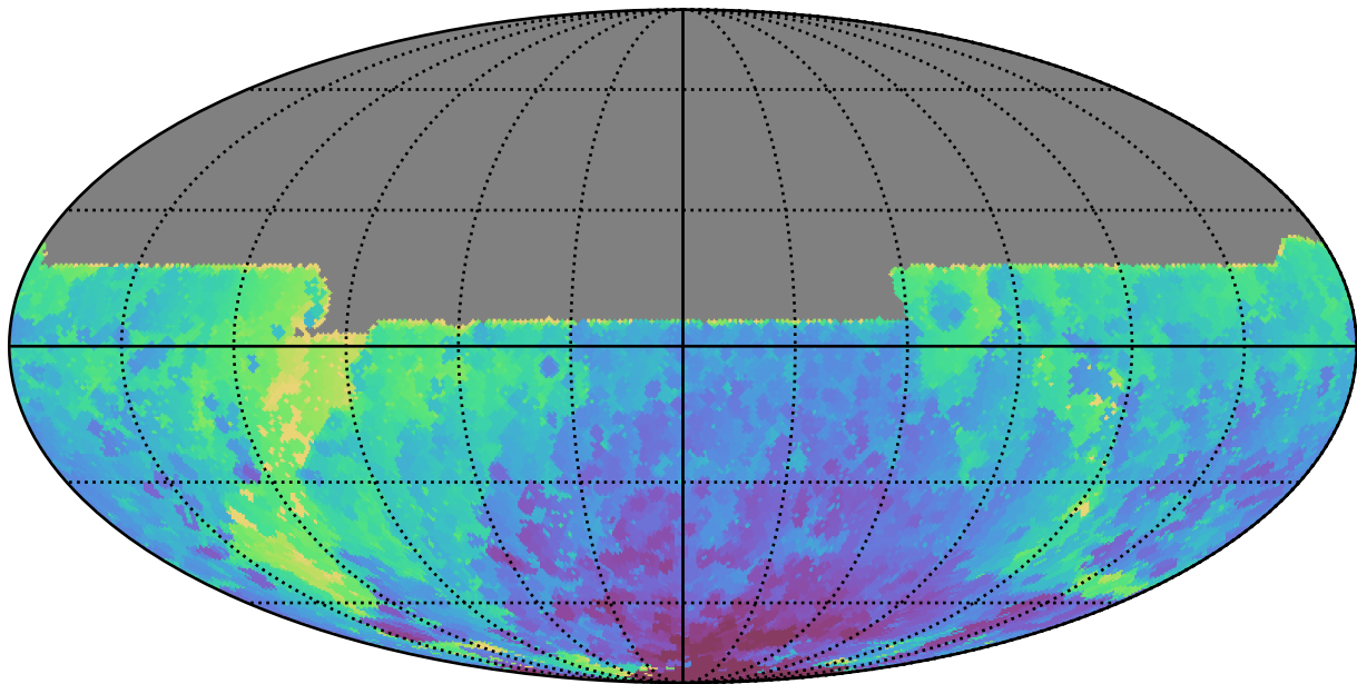
too_elab_r64_d3_griz_v3.4_10yrs All sky y band: Min HA
