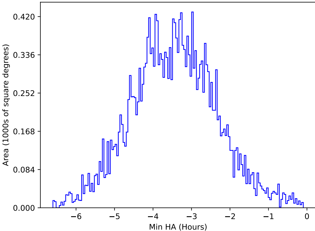
too_elab_r64_d3_griz_v3.4_10yrs All sky y band: Min HA
