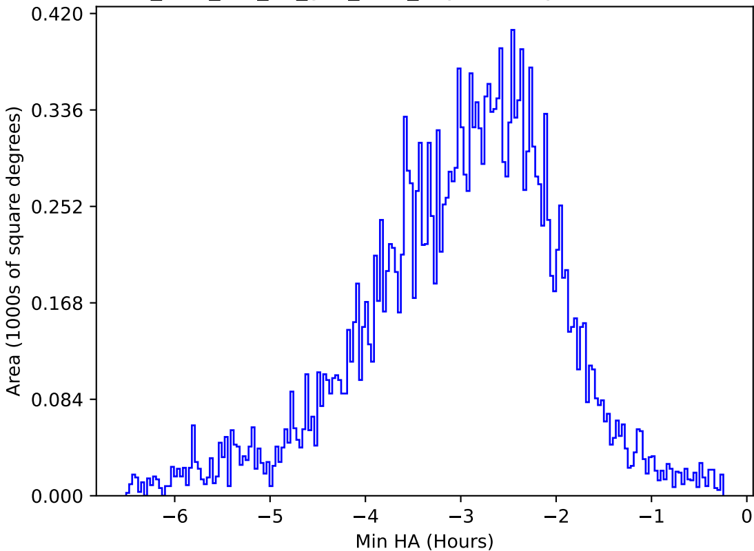
too_elab_r64_d3_griz_v3.4_10yrs All sky u band: Min HA
