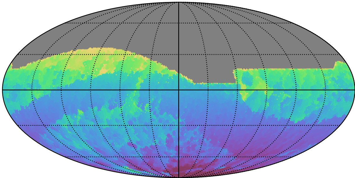
too_elab_r64_d3_griz_v3.4_10yrs All sky r band: Min HA
